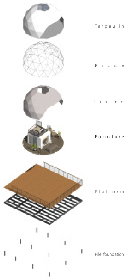
Exploded
